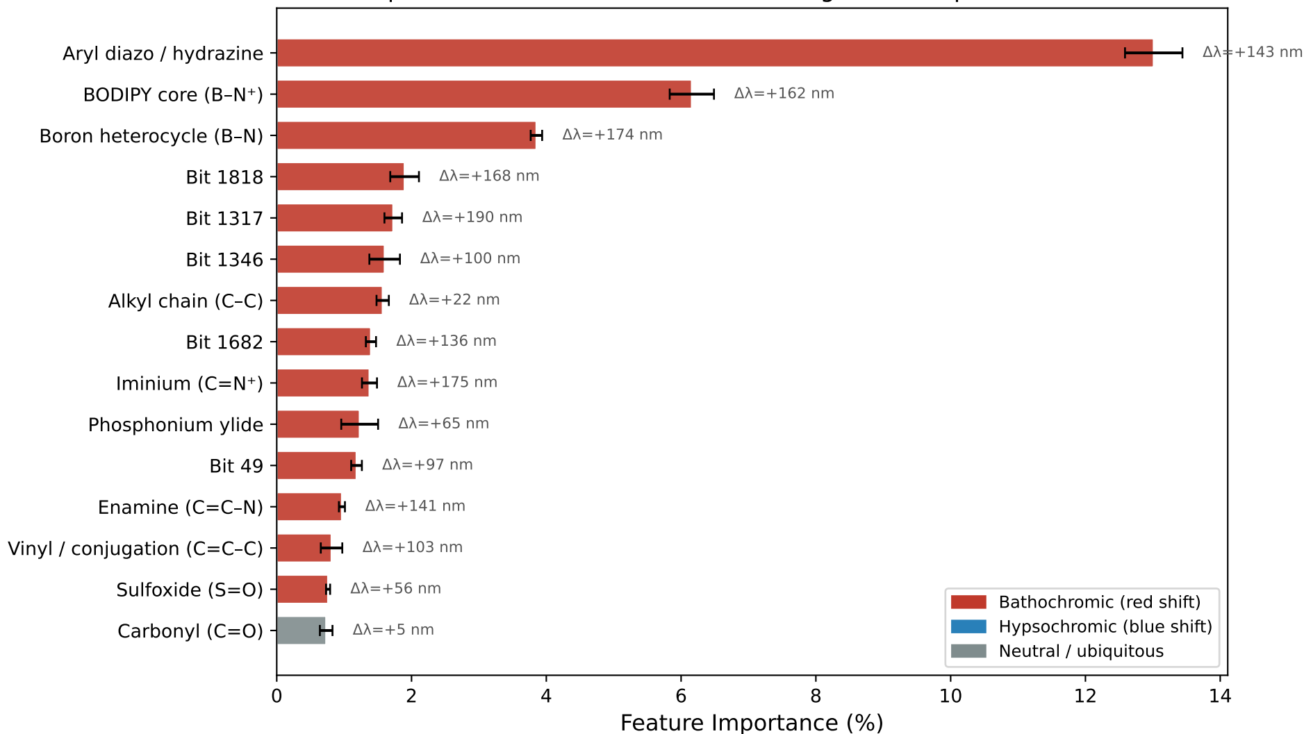
Top 15 Molecular Substructures Driving UV Absorption Prediction
