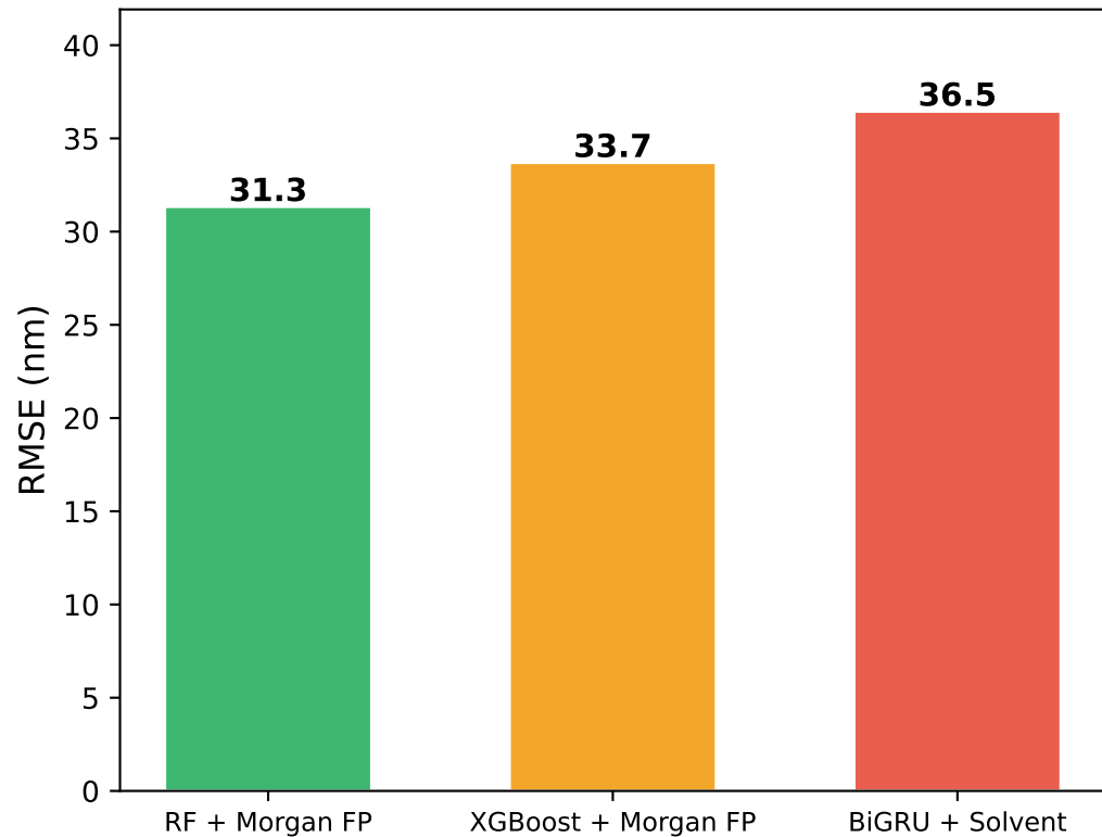
Prediction Accuracy
