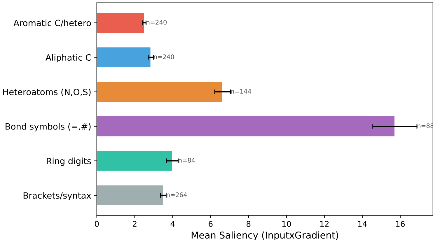
BiGRU Character-Level Saliency by Type (averaged over wetlab molecules)
