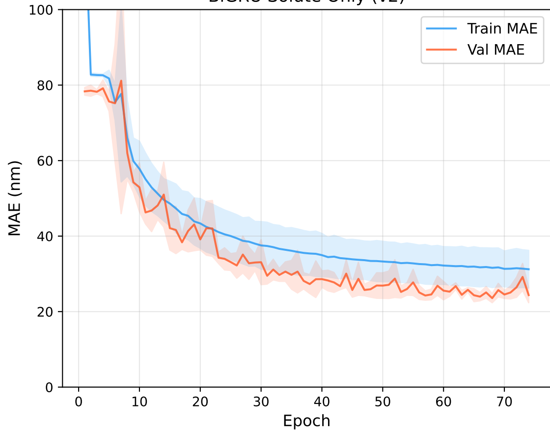
BiGRU Solute Only (v2)
