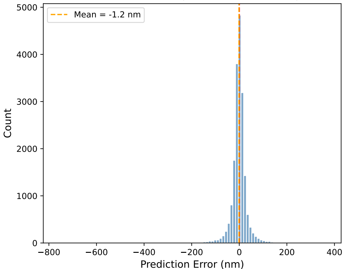
Error Distribution (BiGRU + Solvent, v2)
