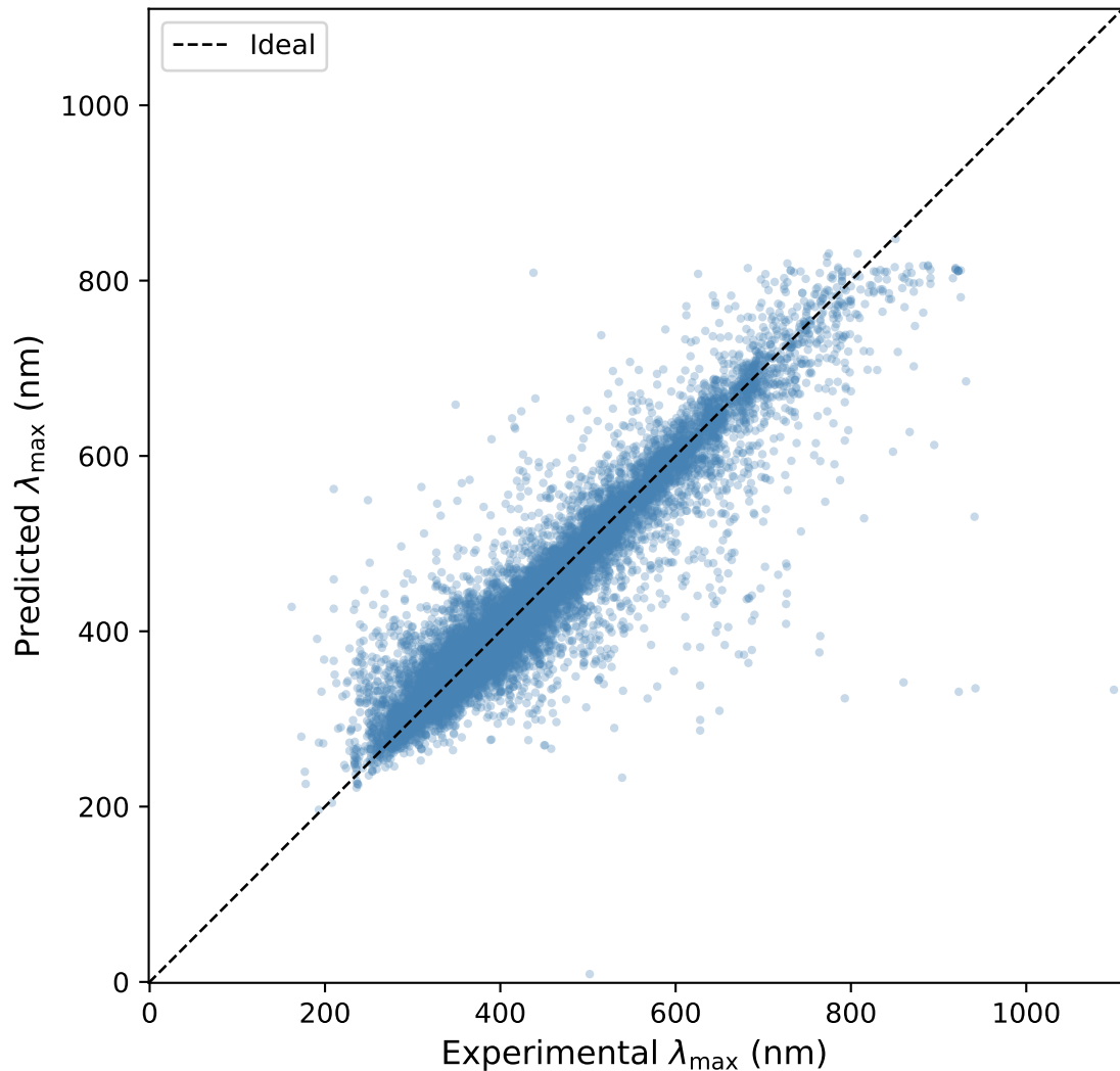
BiGRU + Solvent — 5-Fold CV (RMSE = 36.5 nm)
