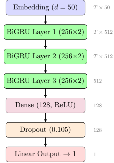
(b) Optimized BiGRU
