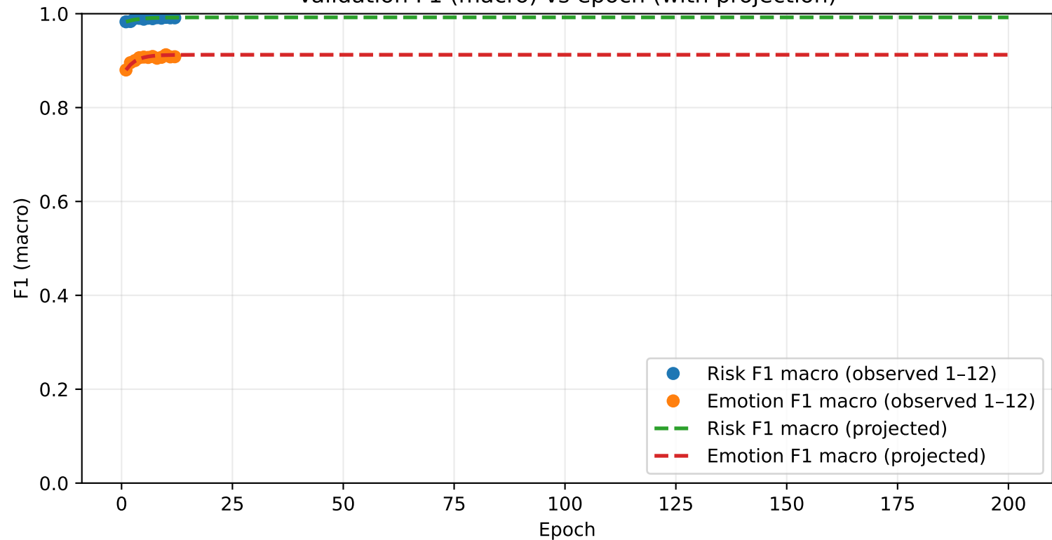
Validation F1 (macro) vs epoch (with projection)
