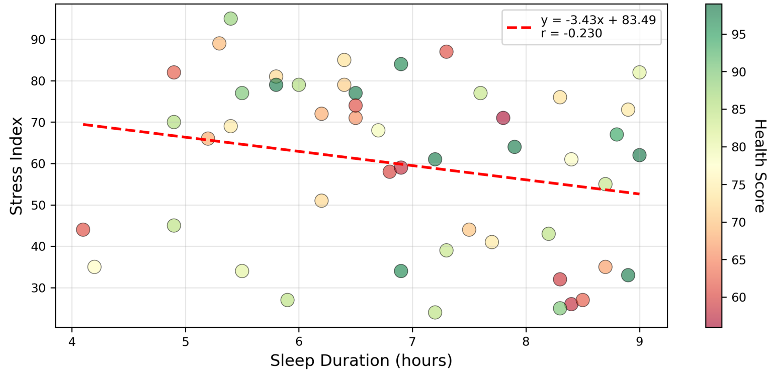
Sleep vs Stress (colored by Health Score)
