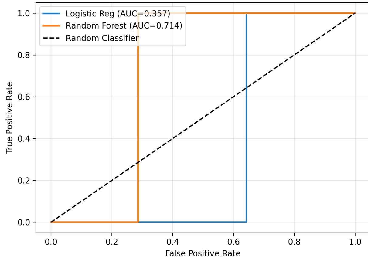
ROC Curves
