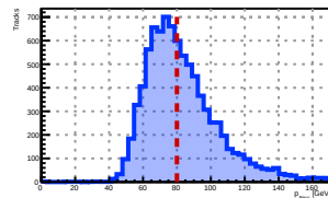
For True Muon Energy 80 GeV
