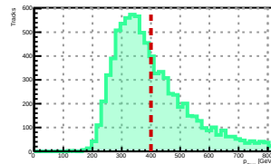
For True Muon Energy 400 GeV
