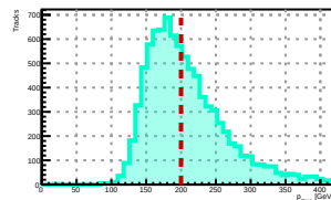
For True Muon Energy 200 GeV
