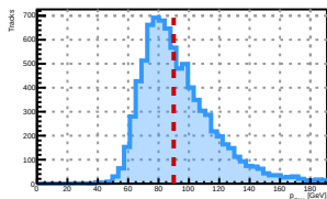
For True Muon Energy 90 GeV
