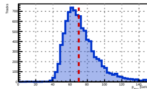
For True Muon Energy 70 GeV
