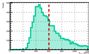
For True Muon Energy 600 GeV
