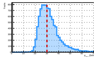
For True Muon Energy 30 GeV
