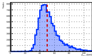
For True Muon Energy 50 GeV
