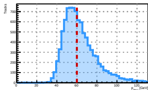
For True Muon Energy 60 GeV
