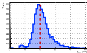
For True Muon Energy 20 GeV
