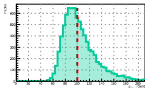
For True Muon Energy 100 GeV
