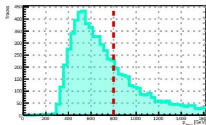
For True Muon Energy 800 GeV
