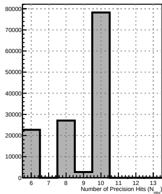
Track Hit Multiplicity Distribution
