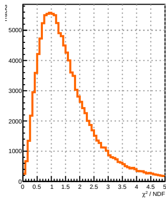
Track Reduced \chi^2 Distribution
