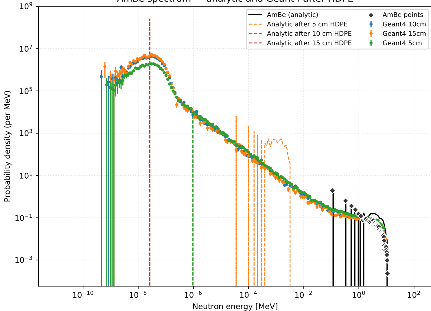
AmBe spectrum — analytic and Geant4 after HDPE
