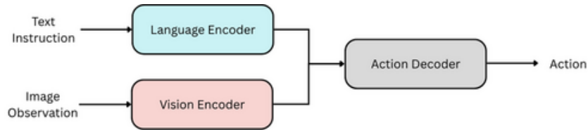
Figure 2.8: Standard vision language action model architecture.
