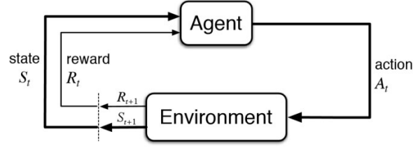
Figure 2.10: Basic RL workflow schema: the agent iteratively maps states to actions by maximizing a cumulative reward signal through trial and error interaction.
