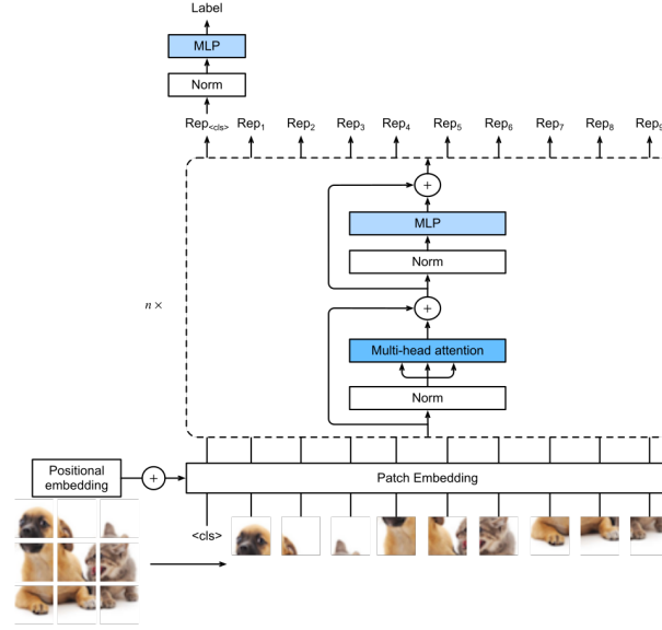
Figure 2.4: Vision transformer architecture
