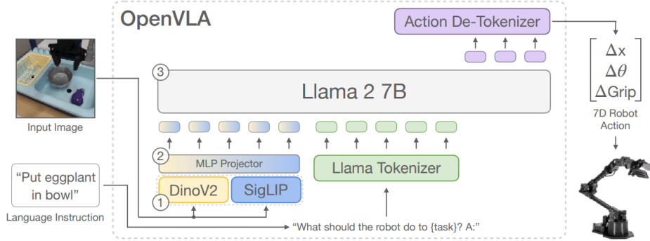
Figure 2.9: Given an image observation and a language instruction, the model predicts 7-dimensional robot control actions. The architecture consists of three key components: a vision encoder, a projector that maps visual features to the language embedding space, and the LLM backbone, in this case, a Llama 2 7B-parameter large language model.
