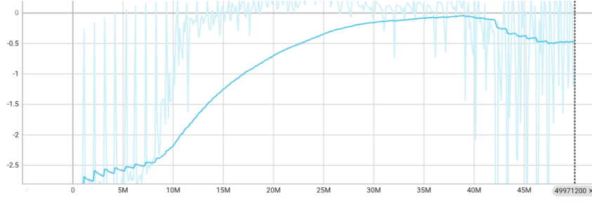
Figure 5.2: Tensorboard train/explained_variance graph progression over near 50M steps.
