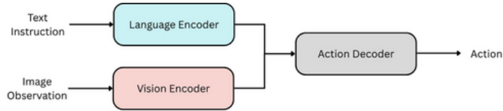
Figure 2.9: Standard vision language action model architecture.
