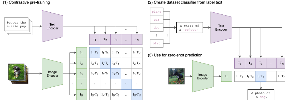
Figure 2.6: CLIP workflow
