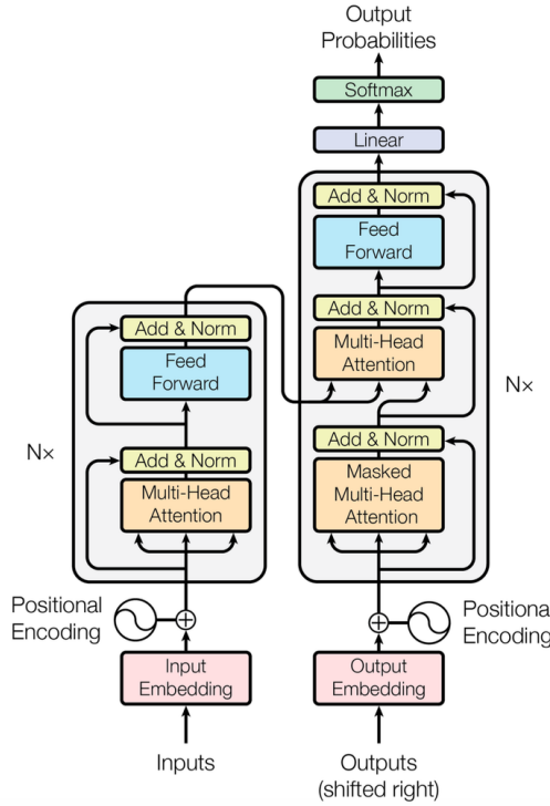
Figure 3.3.: Original Transformers architecture published in " Attention is all you need ".
