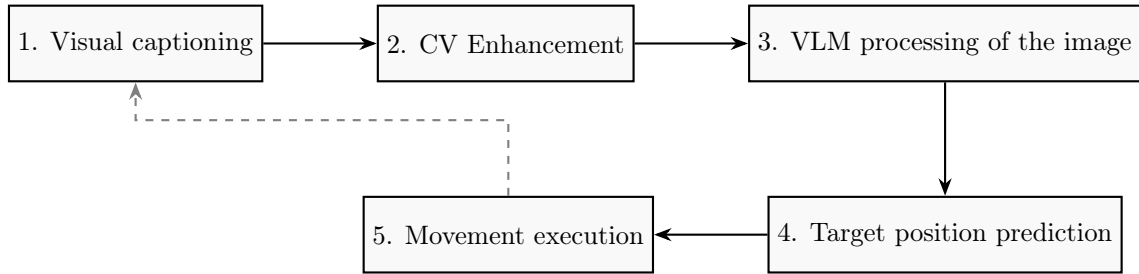
Figure 4.2.: Standard workflow of the solution, going from the visual captioning stage up to the physical agent movement execution. The dashed line indicates a non-continuous feedback loop allowing for cycle repetition, especially in multi-agent tasks.
