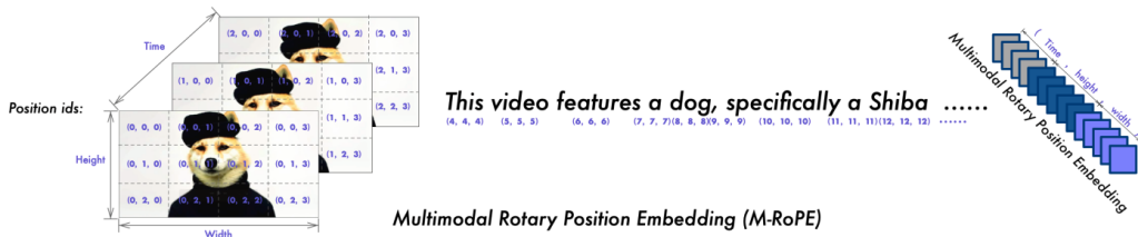
Figure 4.3.: Demonstration of M-RoPE
