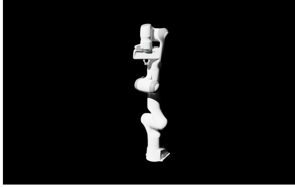
Figure 5.15.: Image of the Franka arm USD, with the 7 original joints plus the added fingers.
