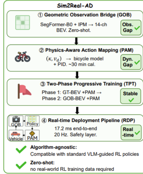
Figure 3.13.: Sim2Real-AD framework’s workflow pipeline illustration.
