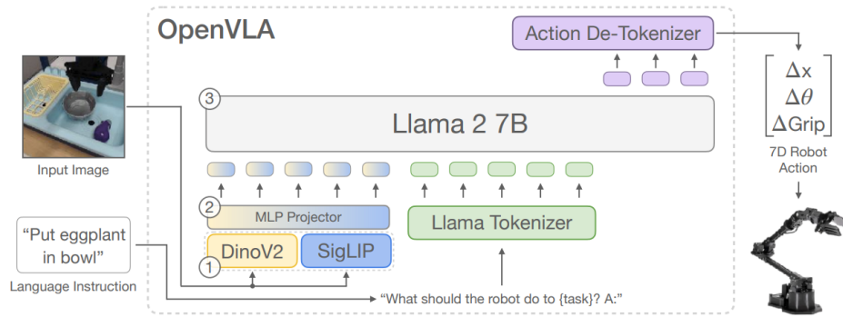
Figure 3.10.: Given an image observation and a language instruction, the model predicts 7-dimensional robot control actions. The architecture consists of three key components: a vision encoder, a projector that maps visual features to the language embedding space, and the LLM backbone, in this case, a Llama 2 7B-parameter large language model.
