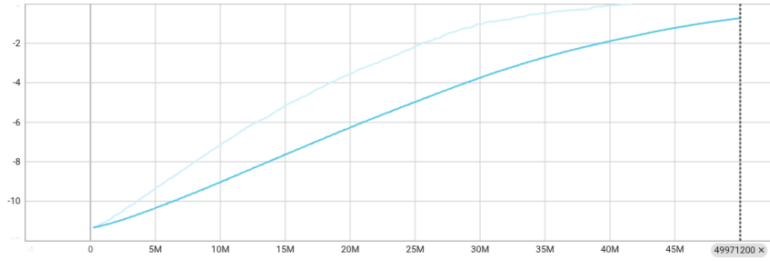
Figure 6.3.: Tensorboard train/entropy_loss graph progression over near 50M steps.
