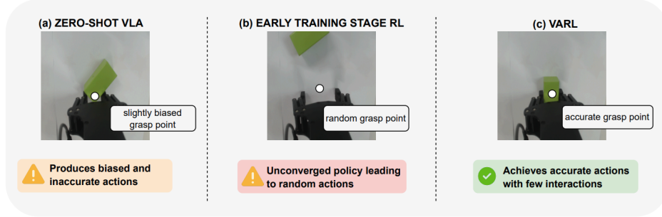
Figure 3.12.: Different RL training approach comparison.
