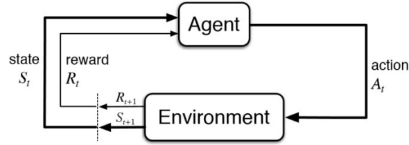
Figure 3.11.: Basic RL workflow schema: the agent iteratively maps states to actions by maximizing a cumulative reward signal through trial and error interaction.
