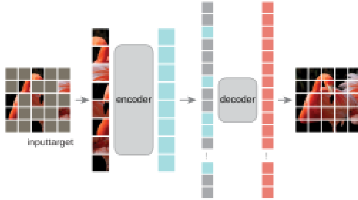
Figure 3.6.: Masked autoencoder architecture.
