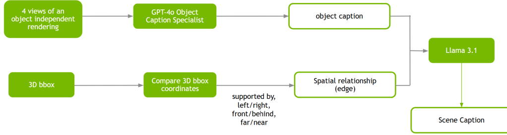
Figure 5.2.: Workflow of the VLM scene captioning add on available at the IsaacSim documentation.
