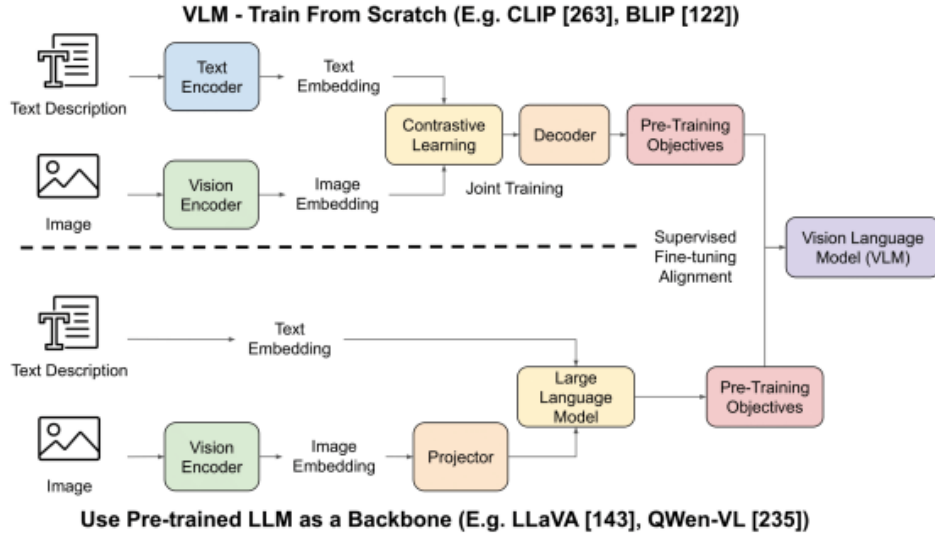
Figure 3.8.: VLM trained from scratch vs training strategy using a pre-trained LLM as backbone.
