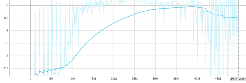
Figure 6.2.: Tensorboard train/explained_variance graph progression over near 50M steps.
