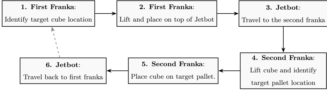
Figure 5.18.: Multi-agent cooperative task workflow. The discontinuous line from step 6 to 1 indicates the able to repeat the cycle once again, as the task may consist on transporting more than one cube.
