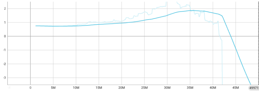
Figure 6.1.: Tensorboard rollout/ep_rew_mean graph progression over near 50M steps.
