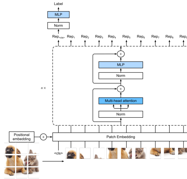
Figure 3.5.: Vision transformer architecture.
