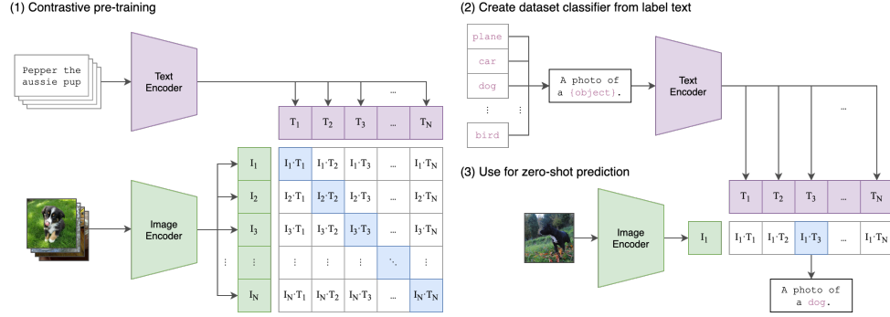
Figure 2.7: CLIP workflow
