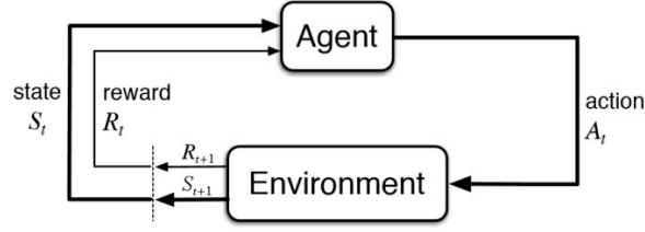
Figure 2.9: Basic RL workflow schema: the agent iteratively maps states to actions by maximizing a cumulative reward signal through trial and error interaction.
