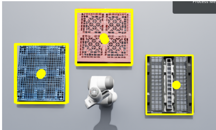
Figure 4.8: Palette detection results with CV application
