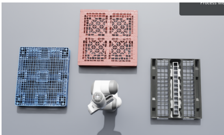
Figure 4.9.: Raw image of pallet detection.
