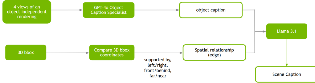
Figure 5.2.: Workflow of the VLM scene captioning add on available at the Isaac Sim documentation.
