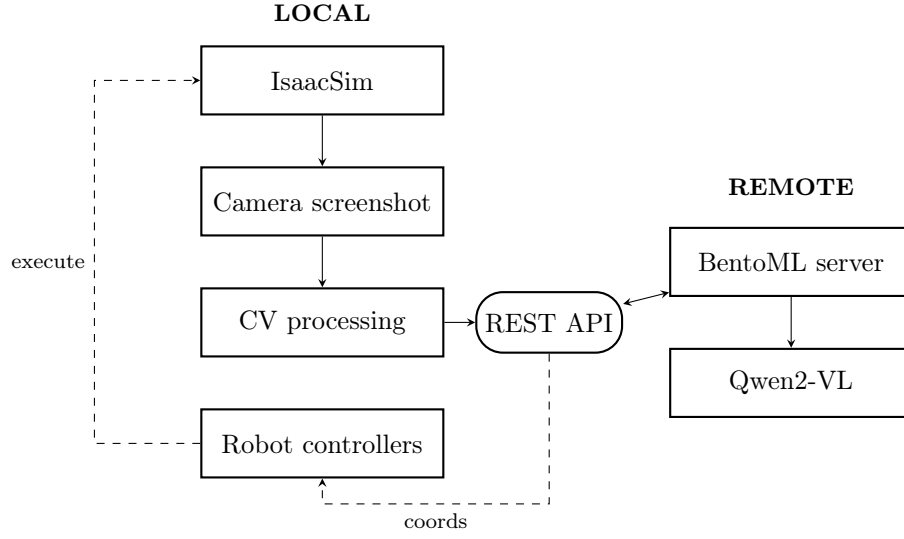
Figure 5.1.: System architecture diagram.
