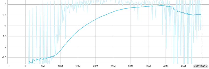
Figure 7.2.: Tensorboard train/explained_variance graph progression over near 50M steps.
