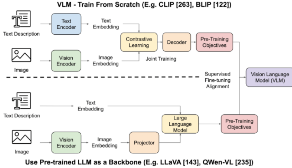
Figure 4.8.: VLM trained from scratch vs training strategy using a pre-trained LLM as backbone.
