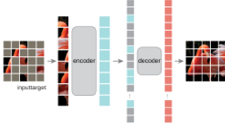
Figure 4.6.: Masked autoencoder architecture.
