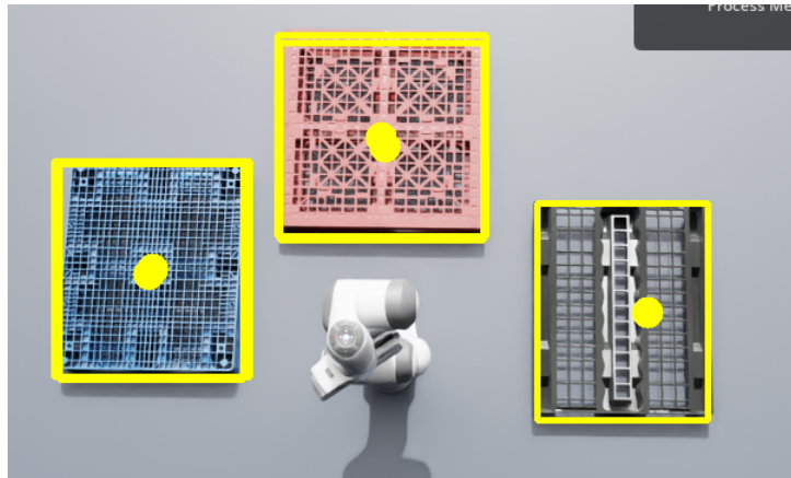
Figure 6.11.: Pallet detection results with CV application.
