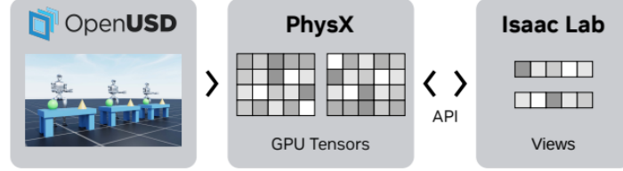
Figure 5.4.: Procedure of how Isaac Lab reads the environment. First converting to tensors the hierarchical representation of the environment, sending them to the GPU and manipulating those tensors via Views API calls.
