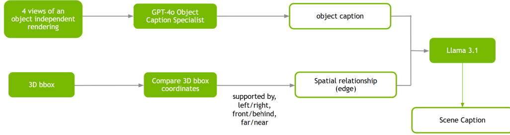
Figure 6.2.: Workflow of the VLM scene captioning add on available at the Isaac Sim documentation.
