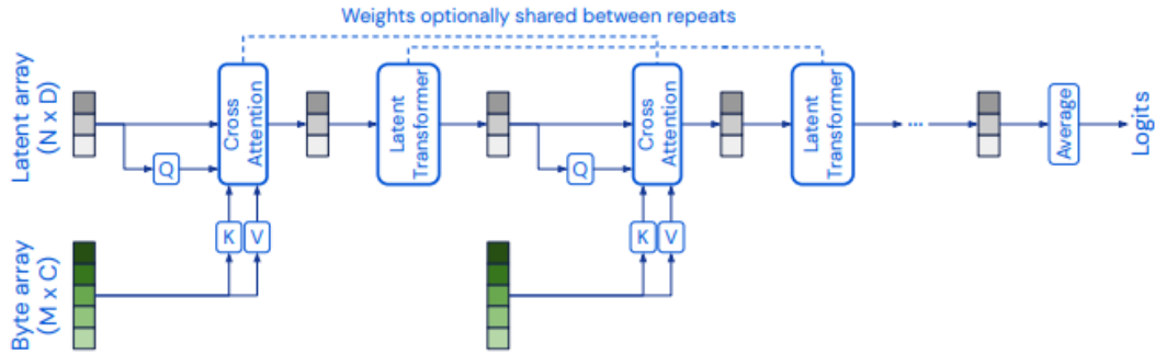
Figure 4.2.: Perceiver architecture from the referenced paper
