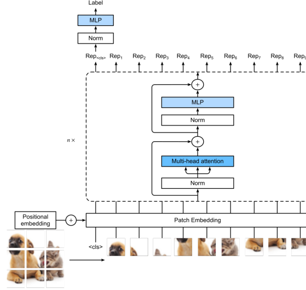
Figure 4.5.: Vision transformer architecture.
