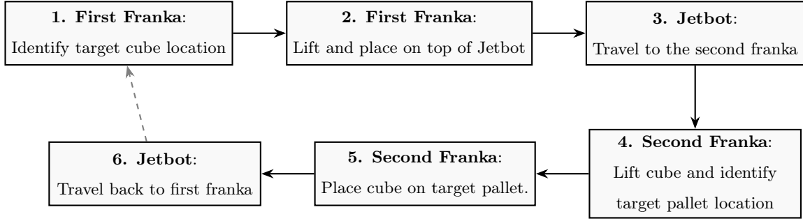
Figure 6.18.: Multi-agent cooperative task workflow. The discontinuous line from step 6 to 1 indicates the able to repeat the cycle once again, as the task may consist on transporting more than one cube.
