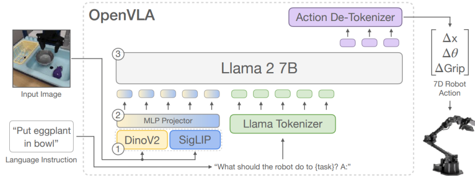
Figure 4.10.: Given an image observation and a language instruction, the model predicts 7-dimensional robot control actions. The architecture consists of three key components: a vision encoder, a projector that maps visual features to the language embedding space, and the LLM backbone, in this case, a Llama 2 7B-parameter large language model.
