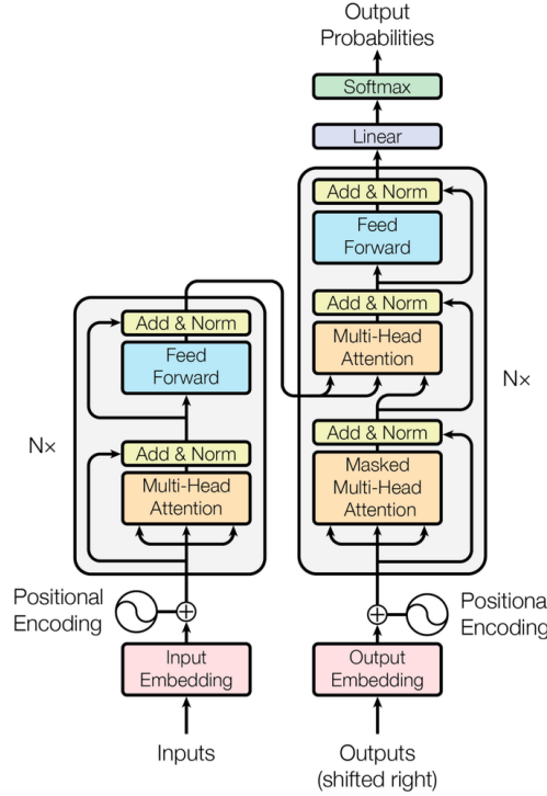
Figure 4.3.: Original Transformers architecture published in " Attention is all you need ".
