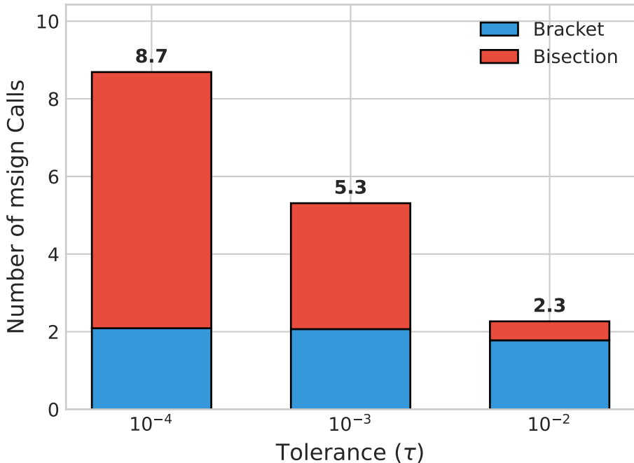
msign Calls Breakdown: Bracket vs Bisection
