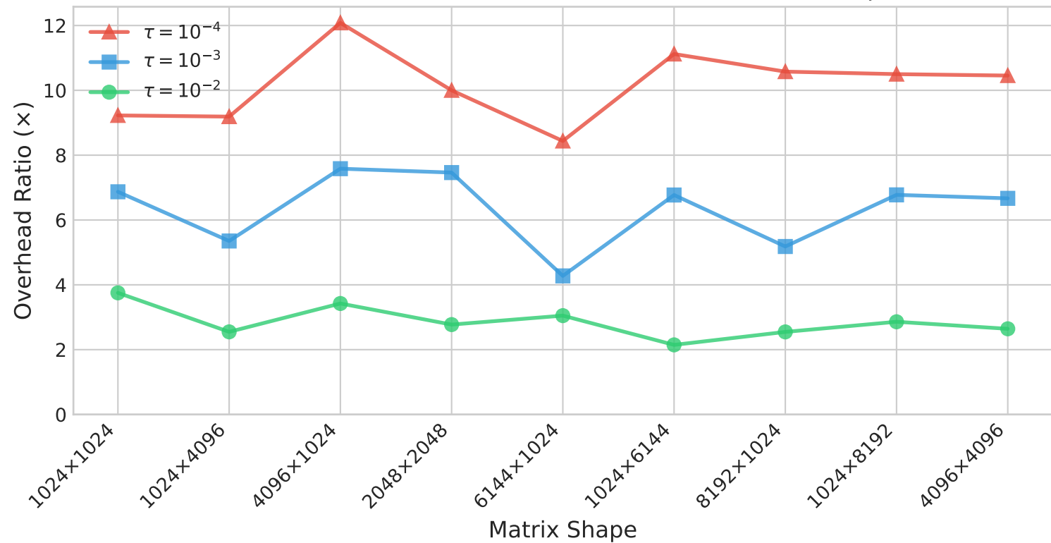
Lambda Solver Overhead Across Different Matrix Shapes
