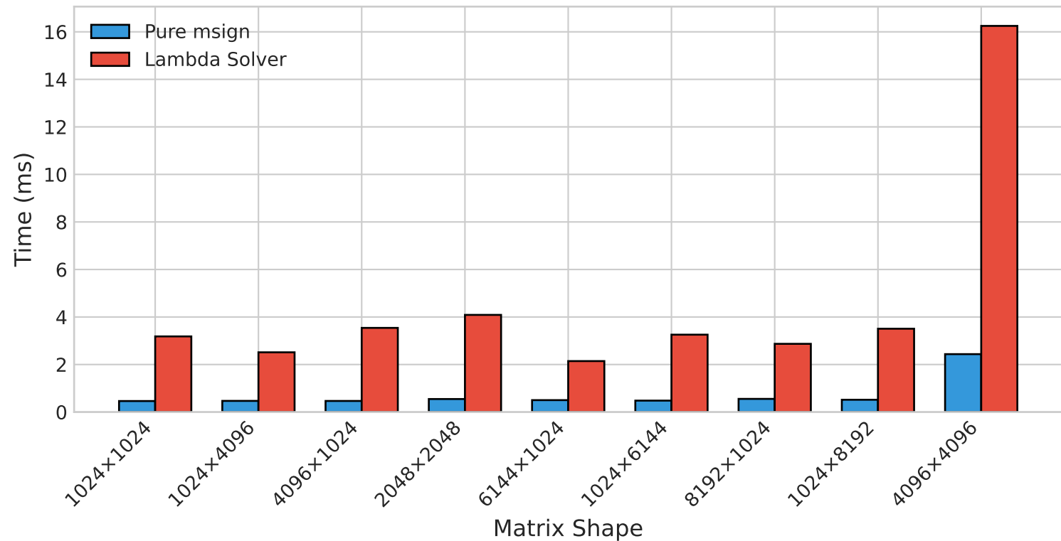
Absolute Runtime Comparison ( \tau = 10^{-3} )
