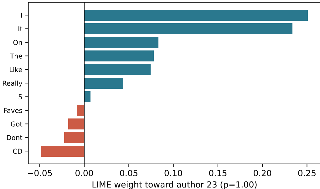
Token contributions for a correctly attributed tweet
