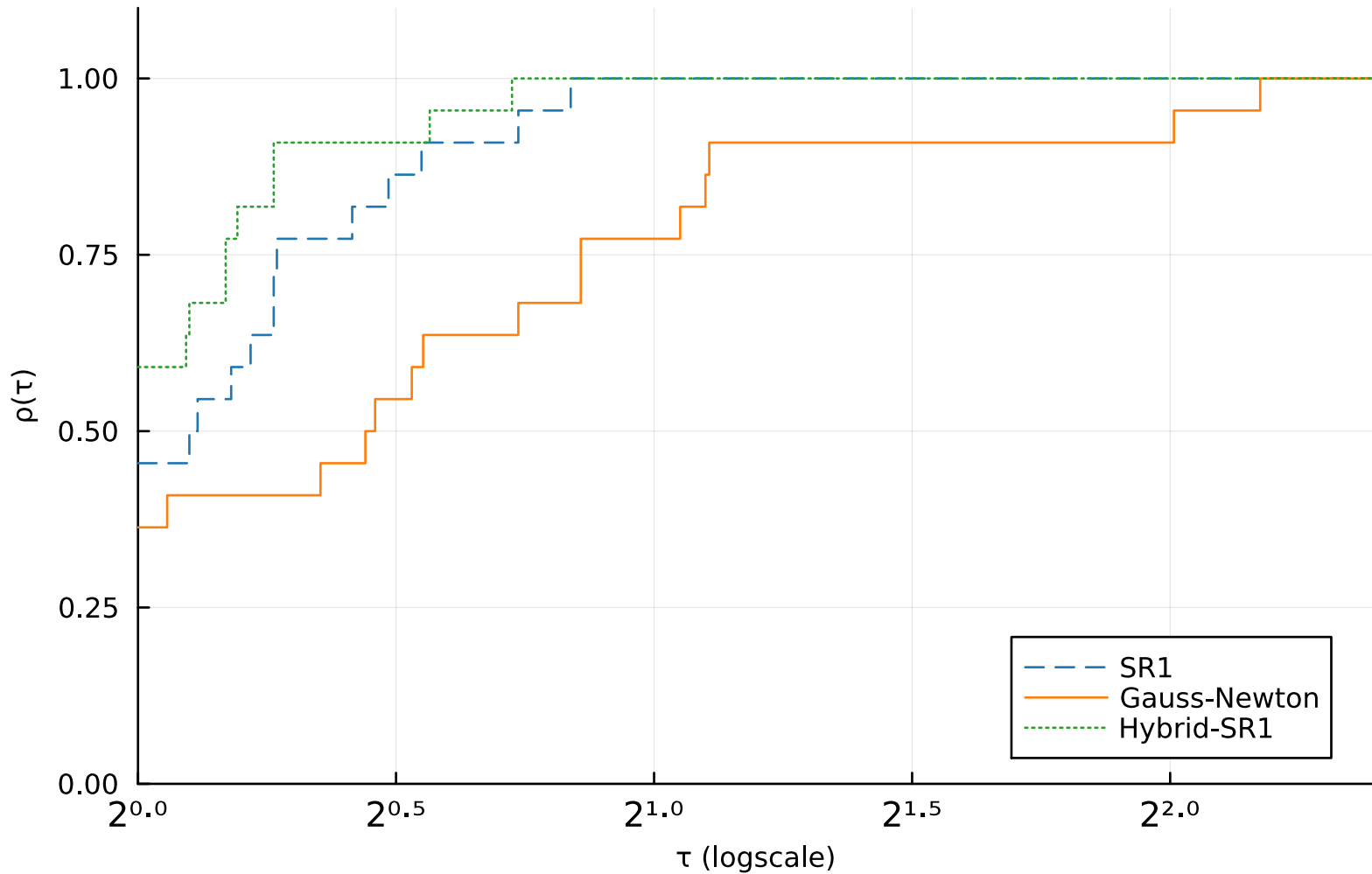
residuals evaluations - 22 problems with 1 \leq ||r_{\text{opt}}||^2 < 100
