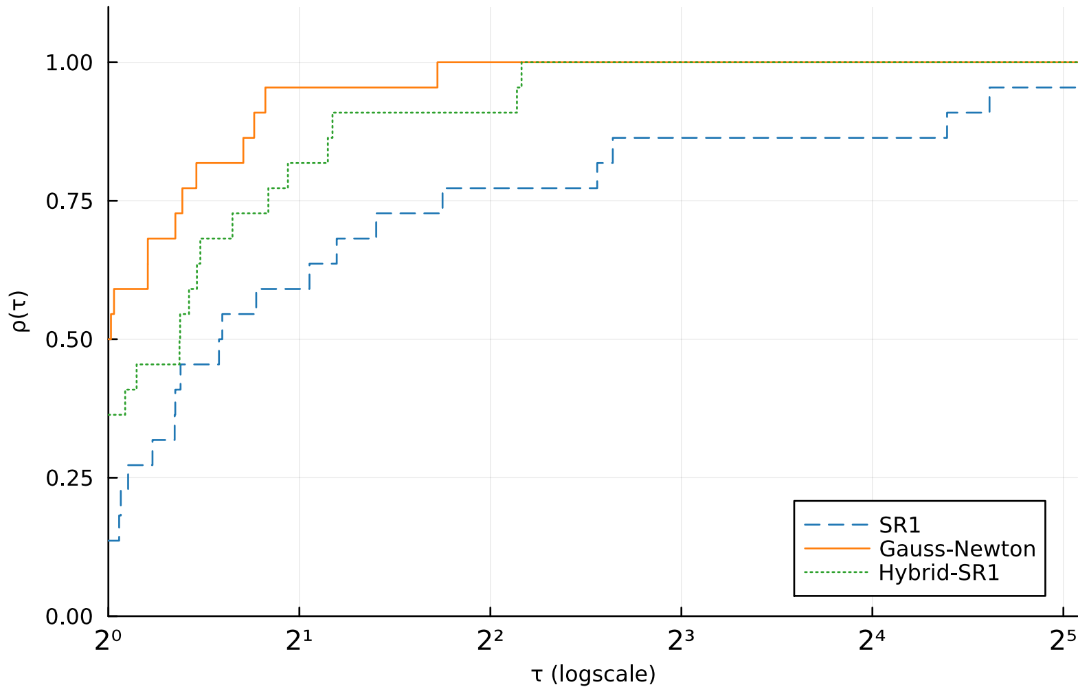
elapsed time - 22 problems with \|r_{\text{opt}}\|^2 \geq 100
