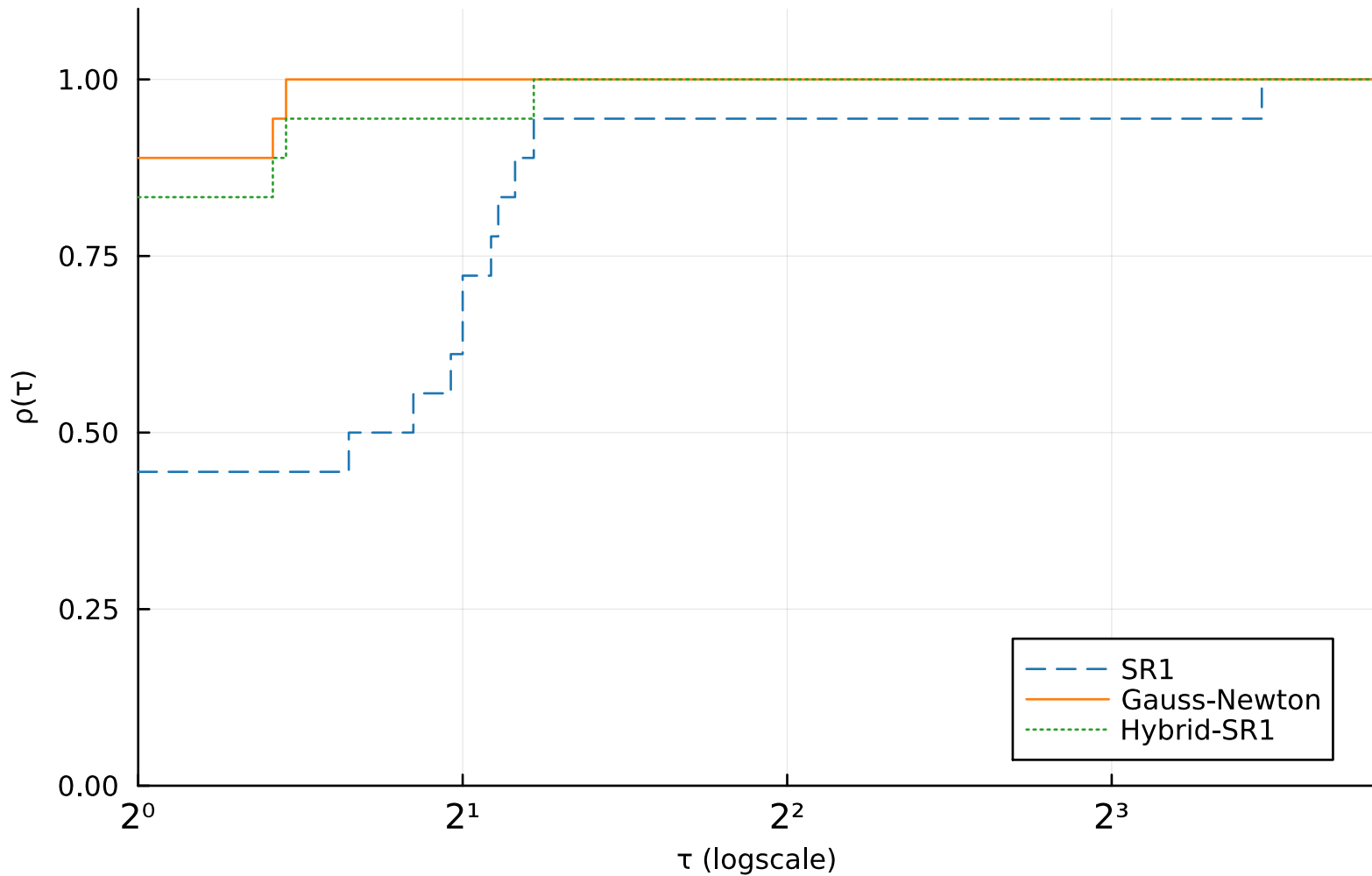
residuals evaluations - 18 problems with \|r_{\text{opt}}\|^2 \leq 10^{-8}
