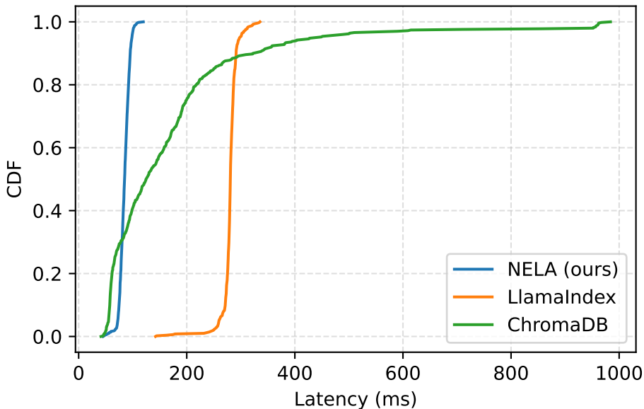
End-to-End Latency CDF
