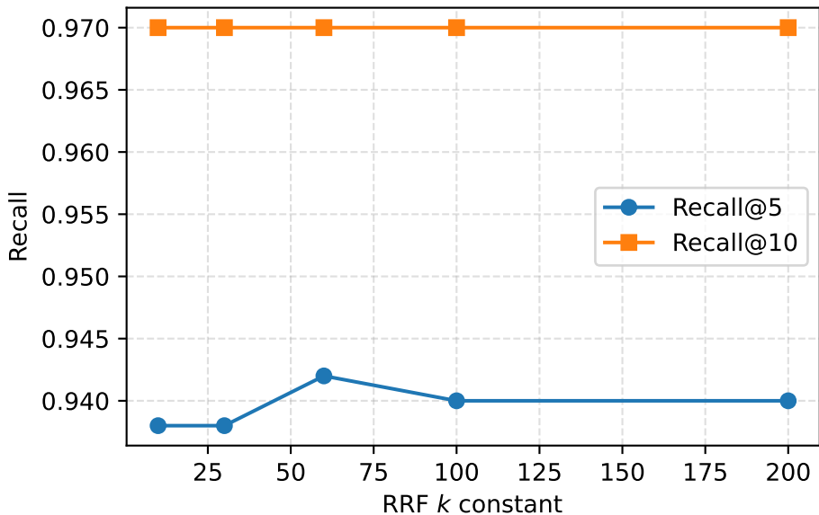
RRF k Ablation
