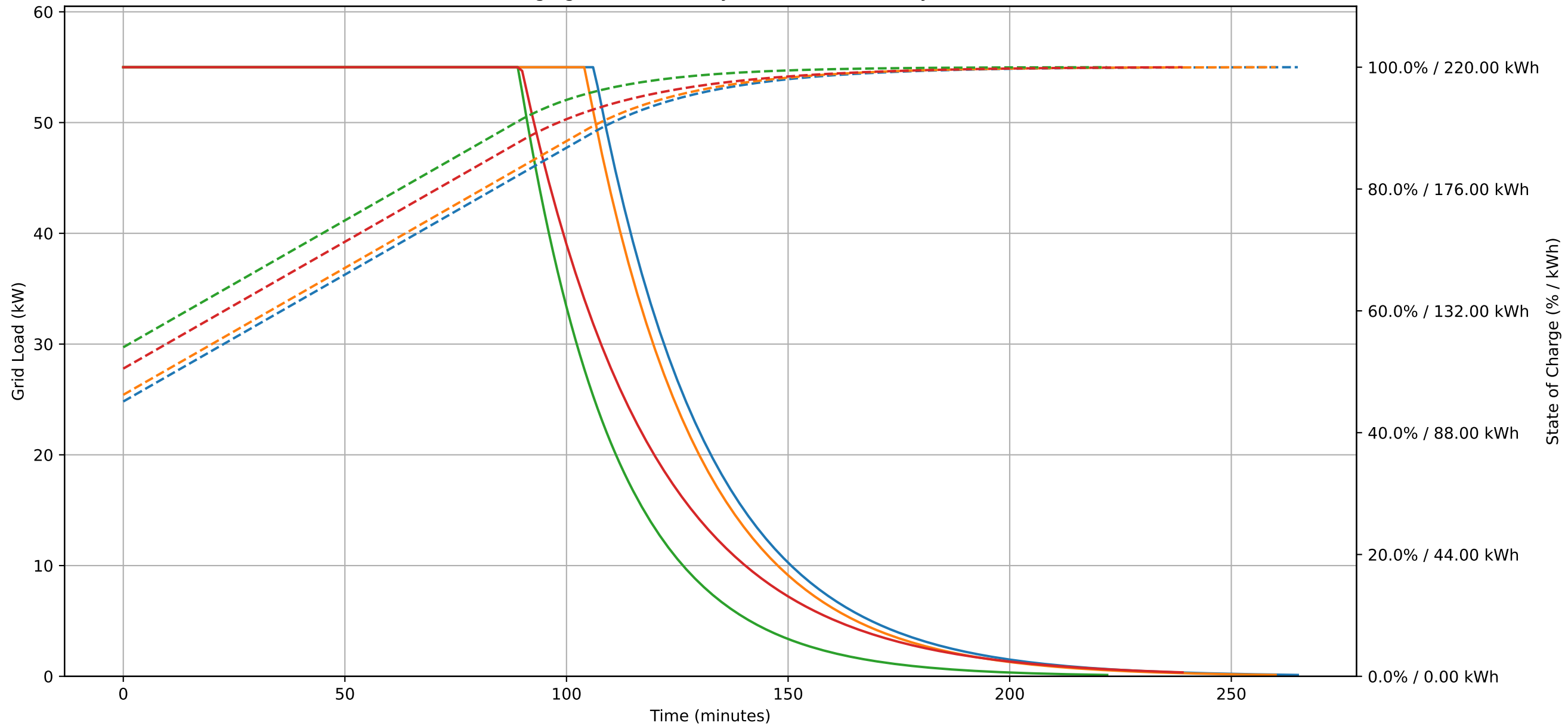
Charging Profiles Overlay for 220 kWh Battery
