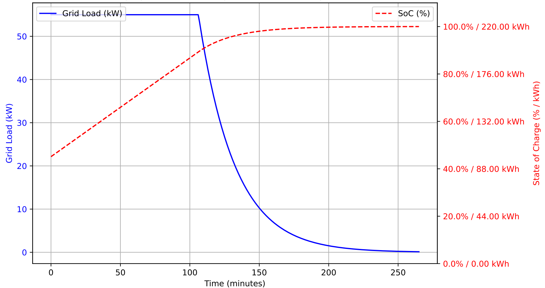
Charging Profile for Config 1: 220 kWh Battery at 0.25C
