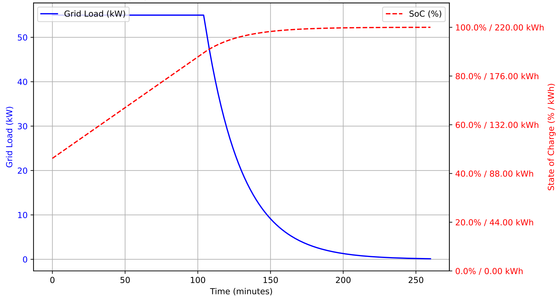
Charging Profile for Config 2: 220 kWh Battery at 0.25C
