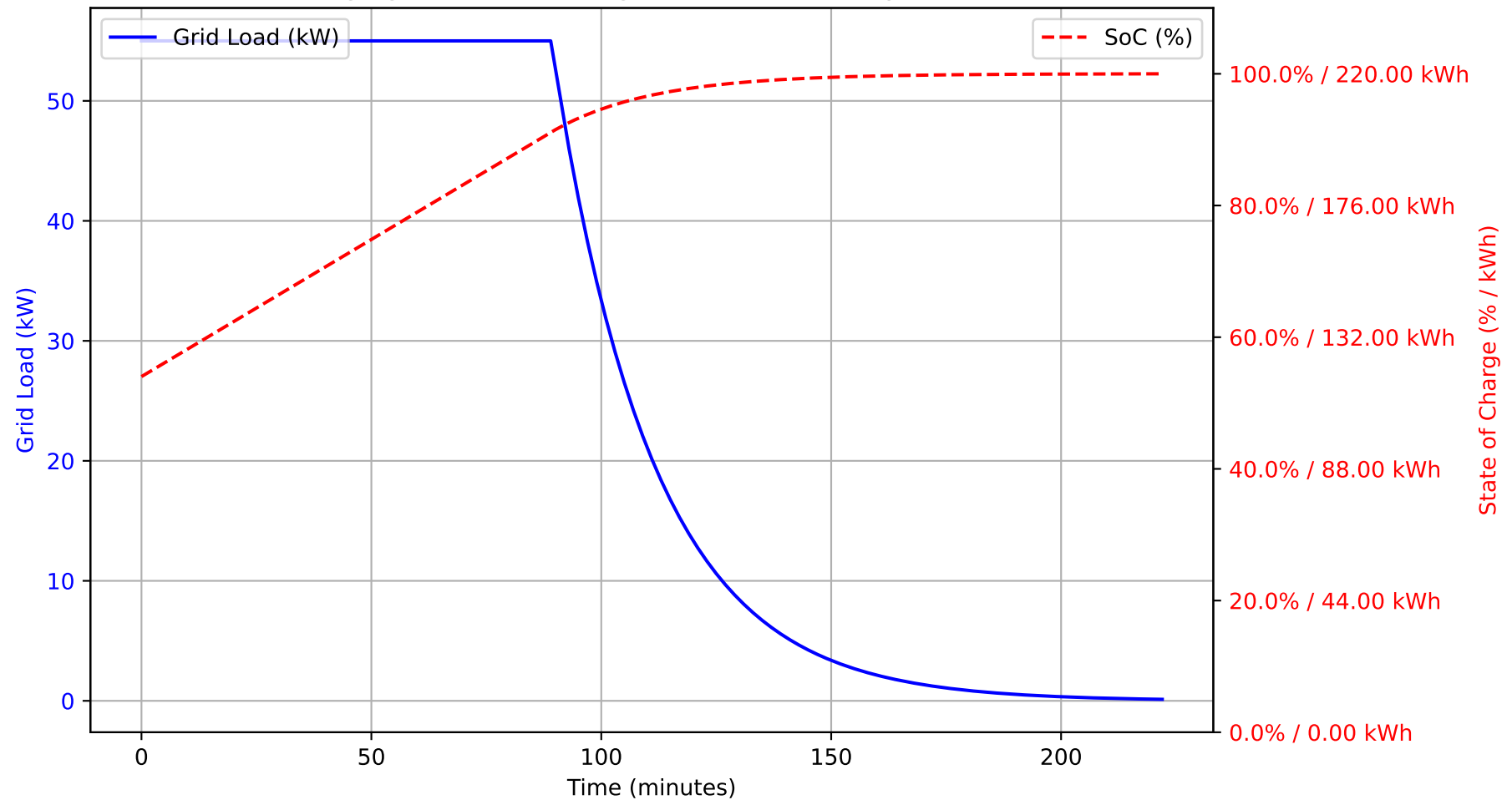
Charging Profile for Config 3: 220 kWh Battery at 0.25C
