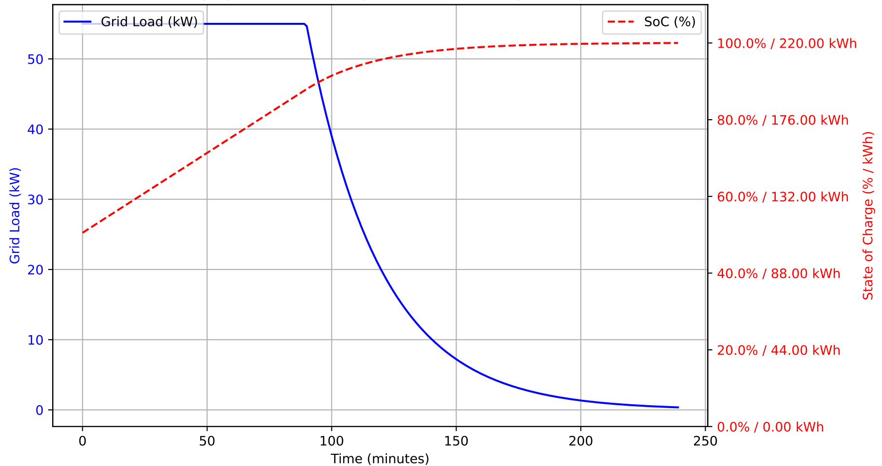
Charging Profile for Config 4: 220 kWh Battery at 0.25C
