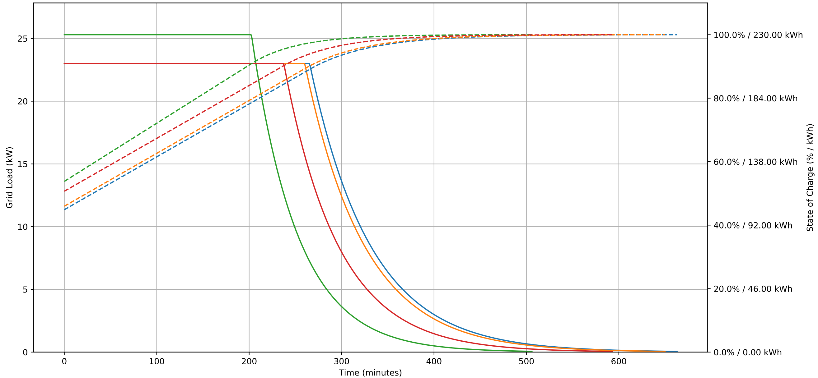
Charging Profiles Overlay for 230 kWh Battery
