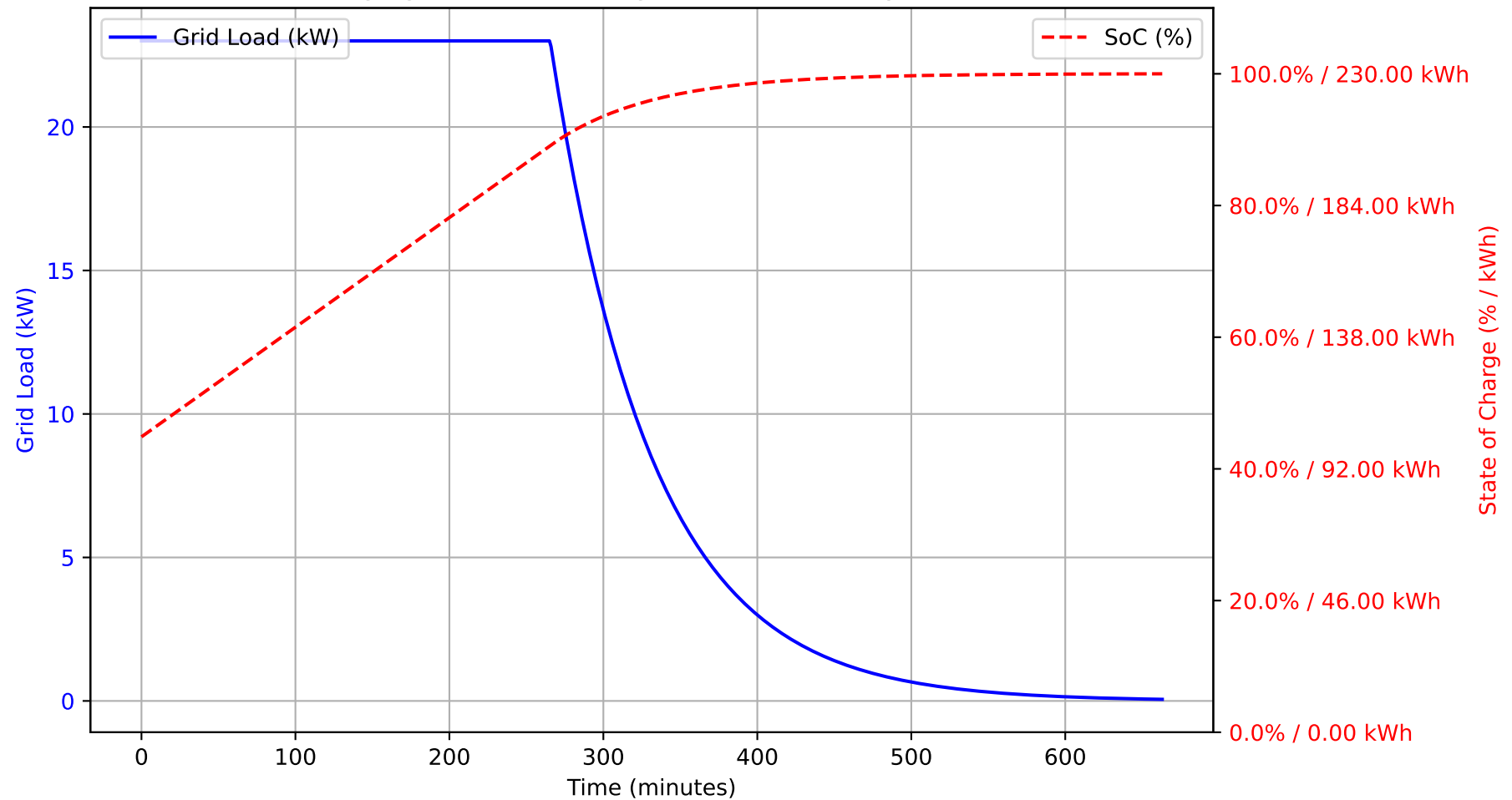
Charging Profile for Config1 230 kWh Battery at 0.1C
