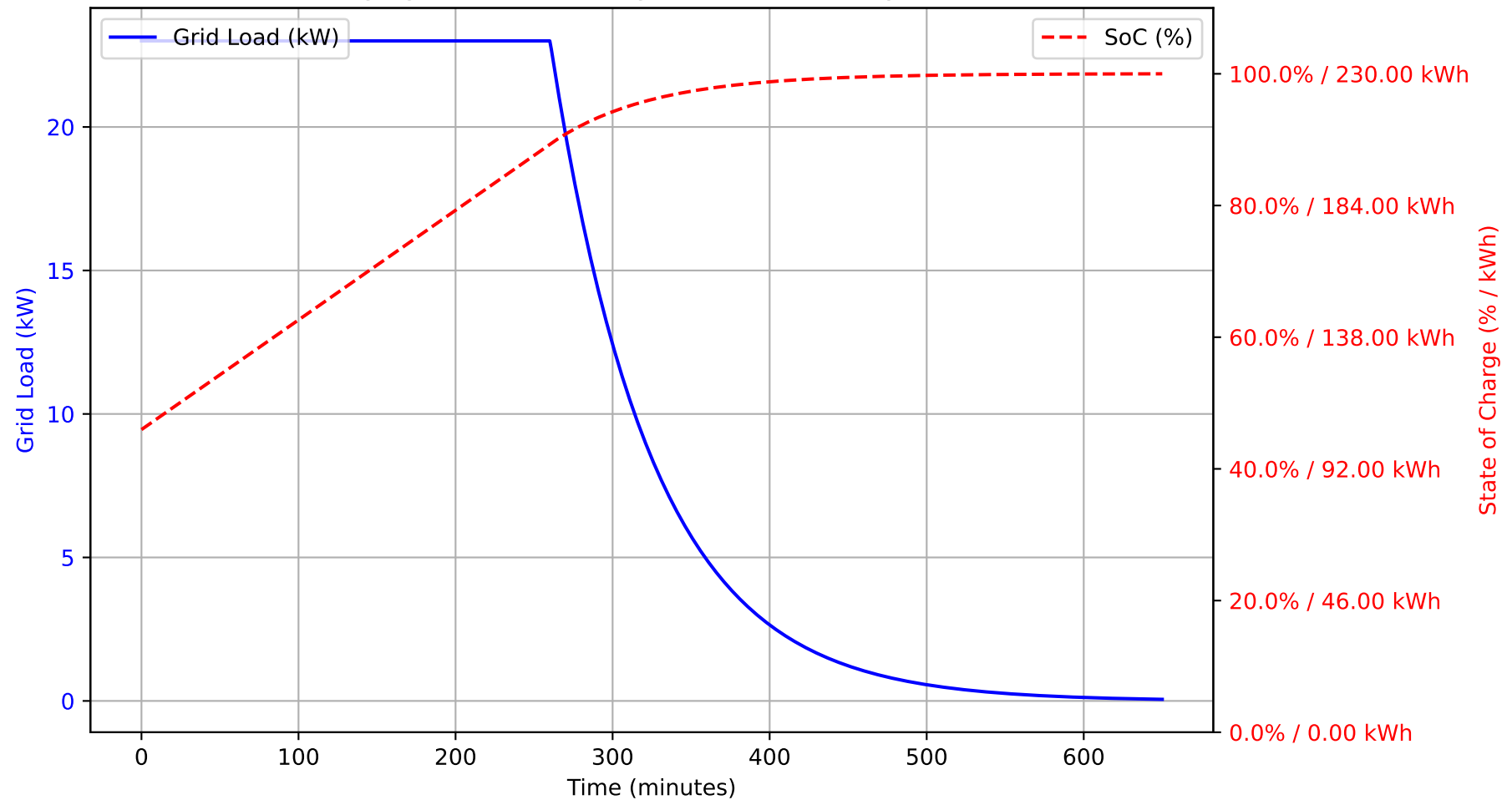
Charging Profile for Config2 230 kWh Battery at 0.1C
