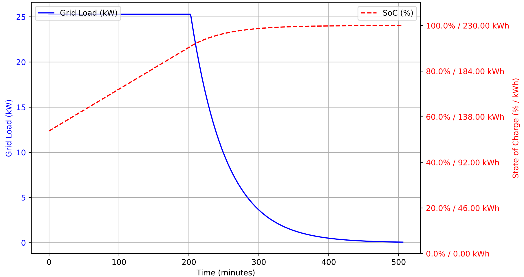
Charging Profile for Config3 230 kWh Battery at 0.11C
