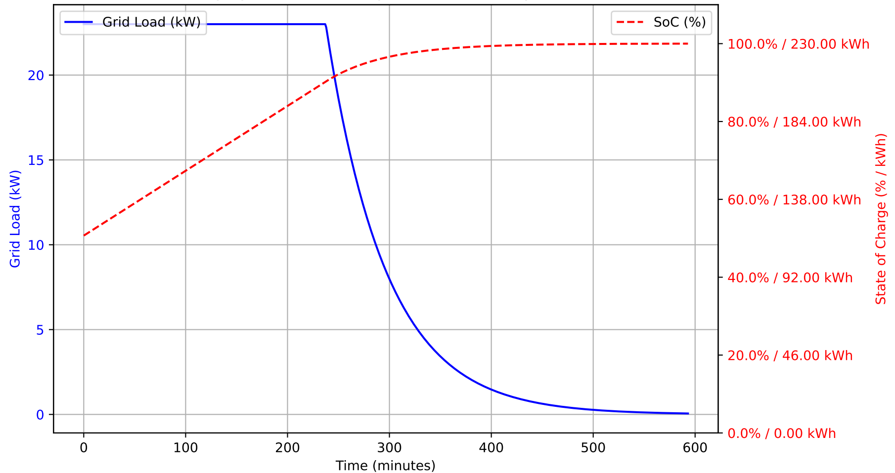
Charging Profile for Config4 230 kWh Battery at 0.1C
