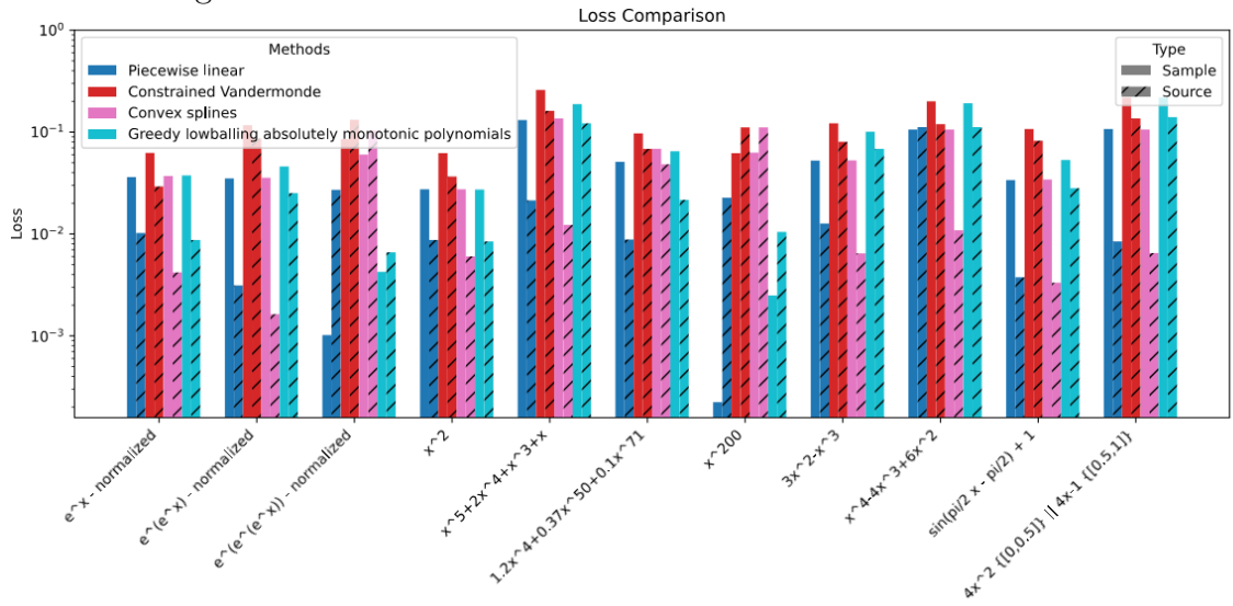
Figure 4: Loss of various methods and source functions
