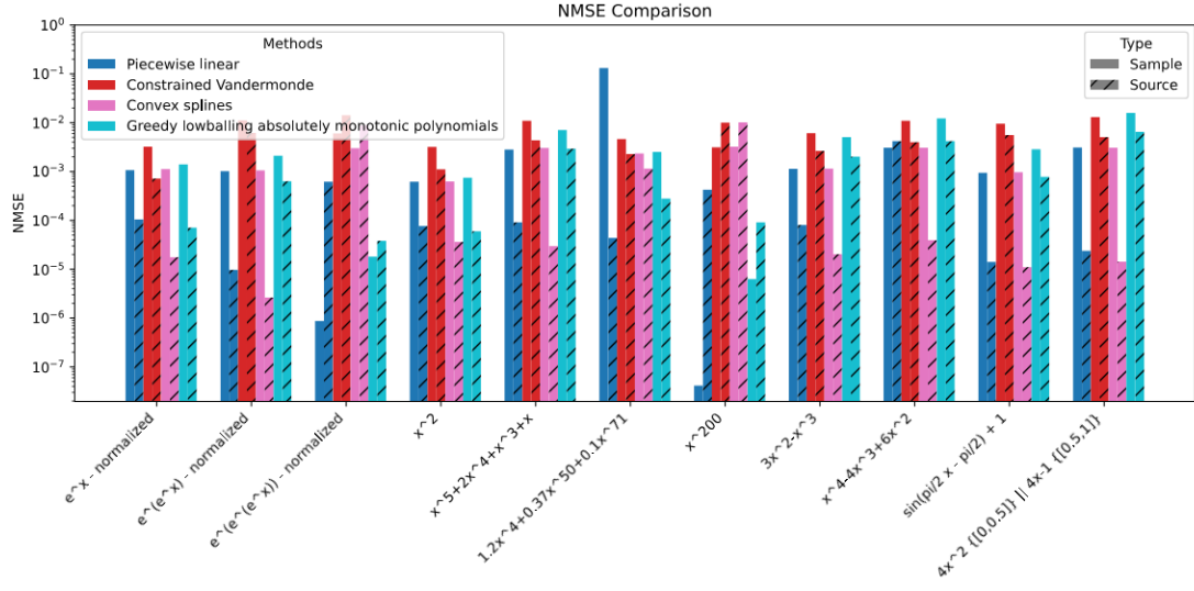
Figure 3: Normalized mean square error of various methods and source functions
