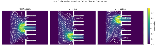
Fig. 6. Flow field comparison for U + M combined mechanism under different channel control configurations. The three sub-figures correspond to middle-, upper-, and lower-channel-controlled setups, respectively. White streamlines and arrows represent time-averaged movement directions; the background color encodes time-averaged density.
