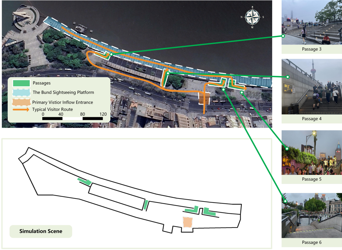
Fig. 10. Real Bund scene and its simplified simulation abstraction. The abstraction retains the Bund sightseeing platform boundary, the main entrance, and the passage connections used for control validation. The satellite basemap was obtained from Google Maps. The right-side local photographs were shot in the Shanghai Bund waterfront passage area by the Tongji Public Safety Experimental Team, June 21, 2026.
