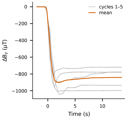
b Cycle overlay (n = 5)
