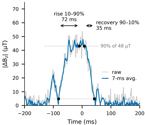
a Tap response event (manual loading)
