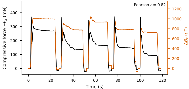
b Five consecutive load-unload cycles (manual loading)
