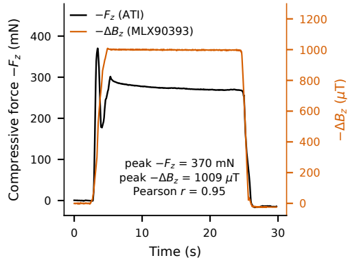
a Single load-hold-unload event (manual loading)
