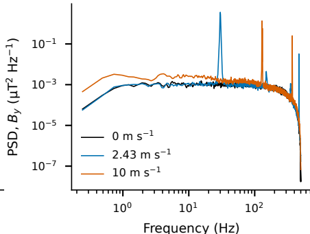
b Narrowband fan harmonics (EMI-confounded) c DC shift tracks time, not speed
