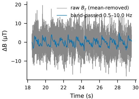
Radial-artery recording, single MLX90393
