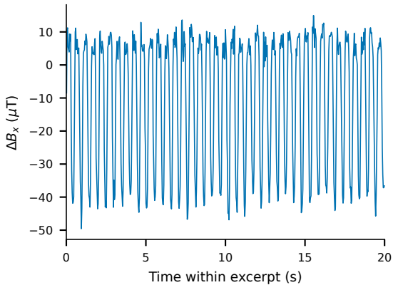
a Raw B_x during cyclic loading (1.95 Hz, 20 s excerpt)
