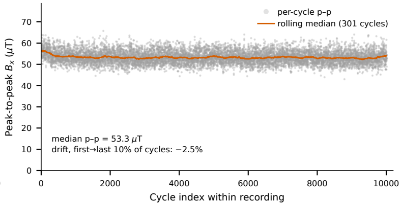
b Within-checkpoint stability ( n = 9,999 cycles)
