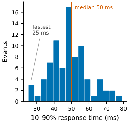
f5 Tap response ( n = 81 )
