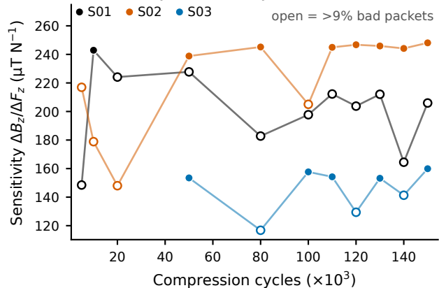
f4 Durability over 150k cycles
